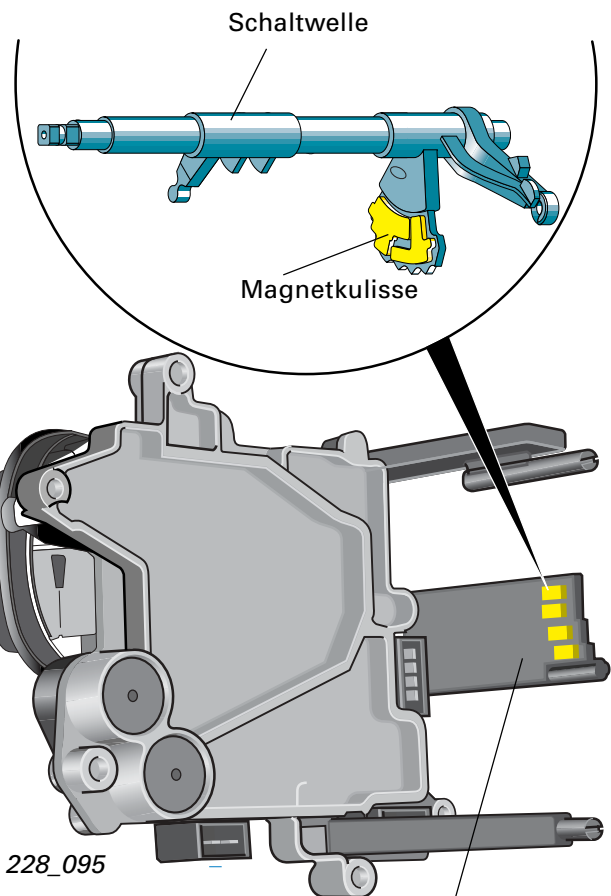
4 Hall-Sensoren A, B, C, D
